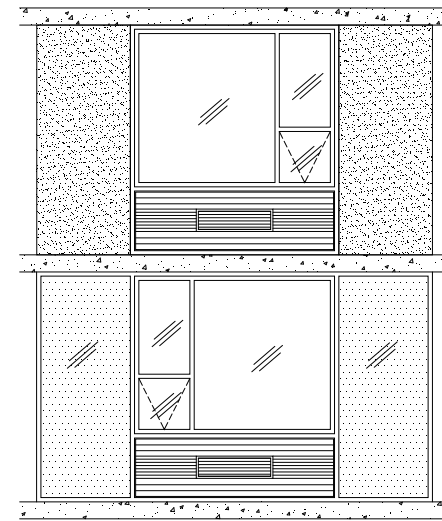
Typical Window Elevation
