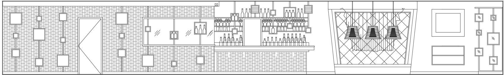
Interior Elevation
